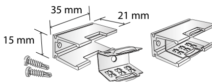
Aluminum mount with clip MC CODE: LS-NF-MC
