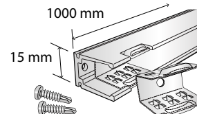
1M Aluminum channel with 2x clip CODE: LS-NF-AP
